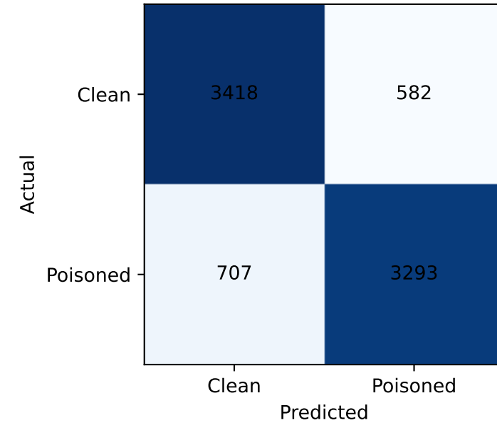
Neural Network
